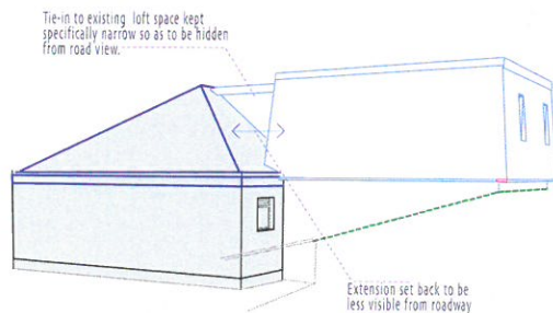
Perspective view from South
